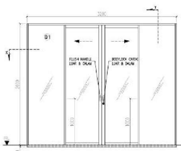
Sliding Pocket 2R4S (Daun Tengah Sliding, Kanan Kiri Mati)
